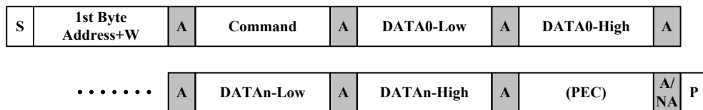
Figure 9-1-2-1. Command write cycle diagram
