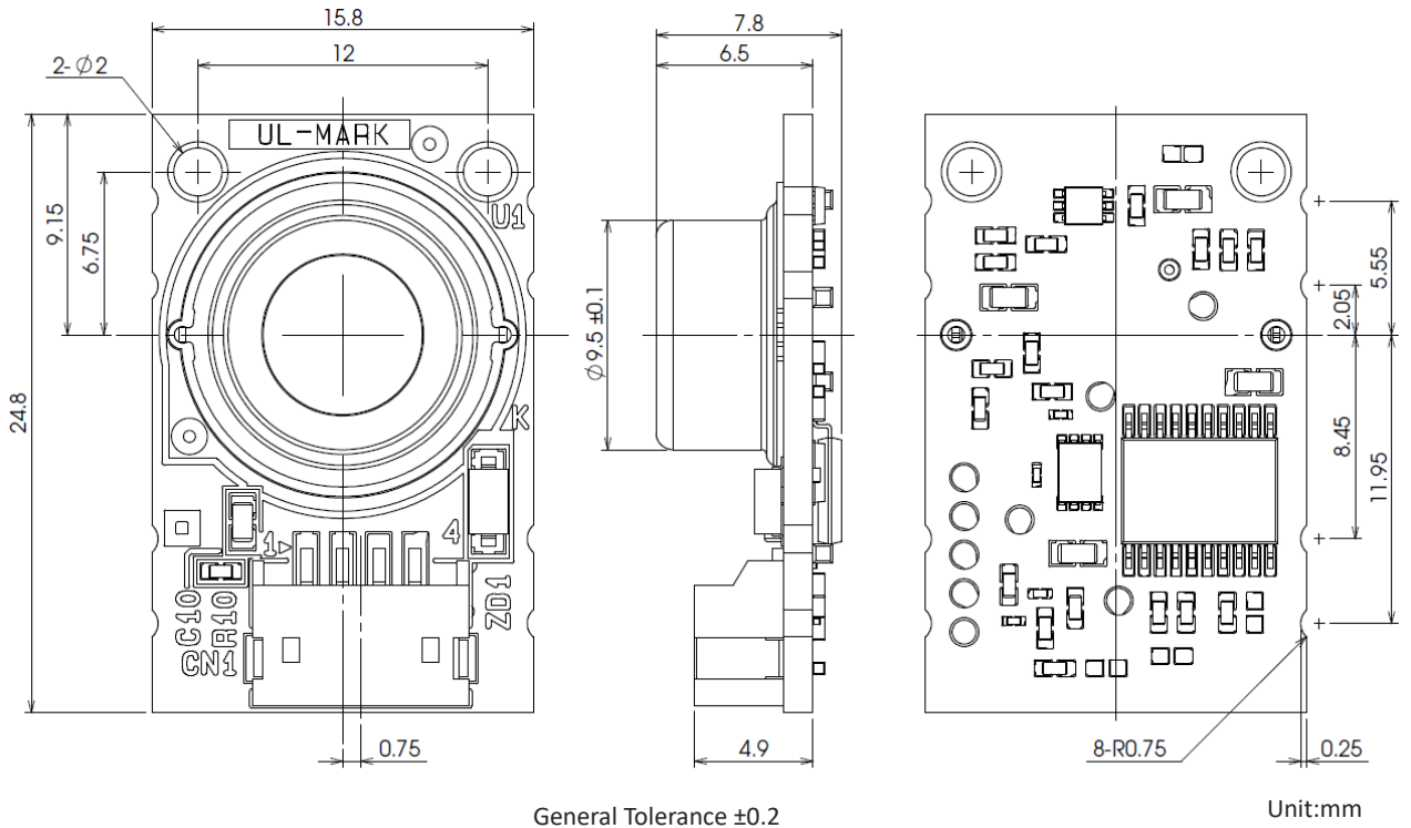
Figure 12-1. External dimensions
