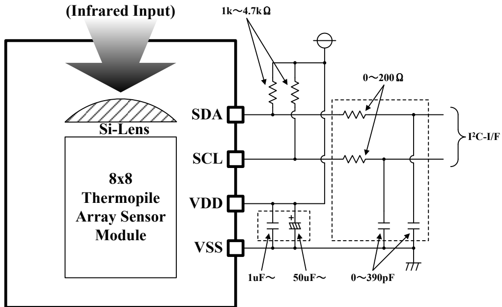
Figure 11-1. Typical application circuit
