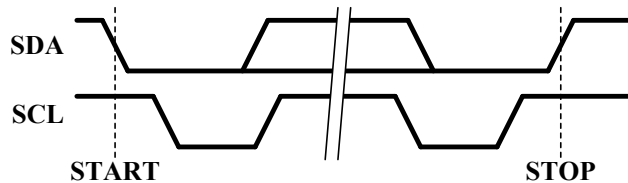
Figure 9-1-1-1. Start/Stop conditions
