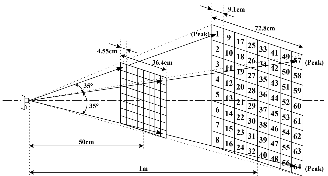
Figure 10-1. Field-of-view image diagram
