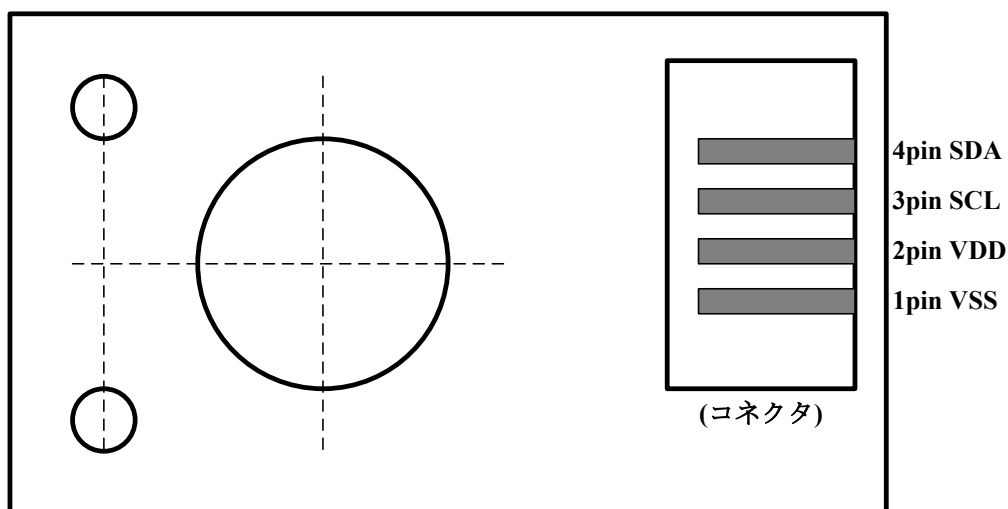
Figure 4-1. Pin layout diagram
