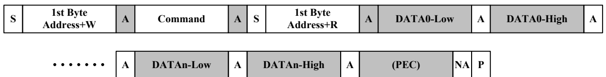
Figure 9-1-2-2. Command read cycle diagram
