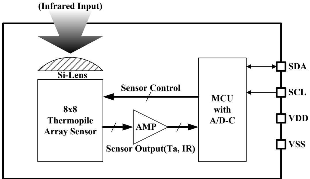
Figure 3-1. Block Diagram
